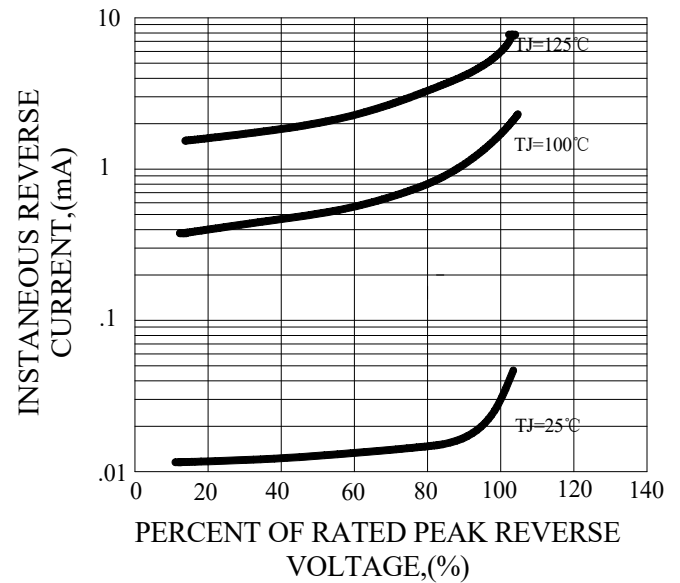
FIG.4-TYPICAL REVERSE CHARACTERISTICS
